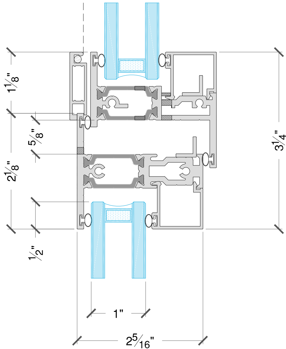
3a Intermediate (Hopper & Fixed)
