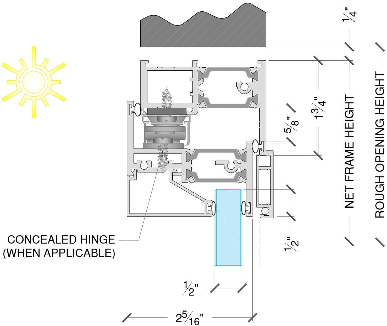
1b Casement Head - No Nail Fin & Monolithic Stop
